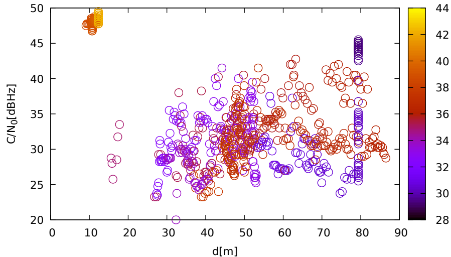
C/N 0 vs distance (JavadLSA at C 3 for G08 at L1)
