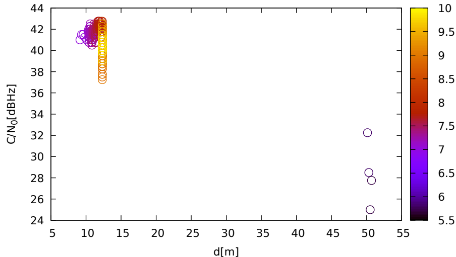
C/N 0 vs distance (JavadLSA at C 3 for G10 at L1)
