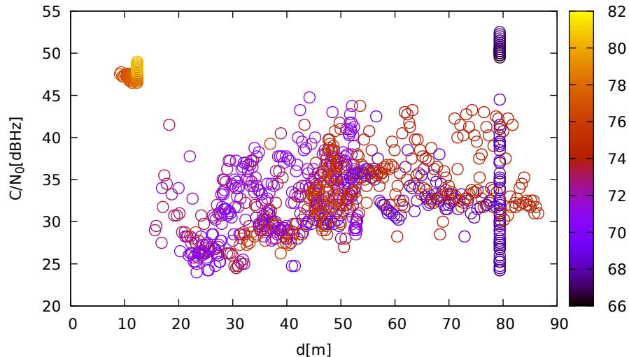
C/N 0 vs distance (JavadLSA at C 3 for G11 at L1)
