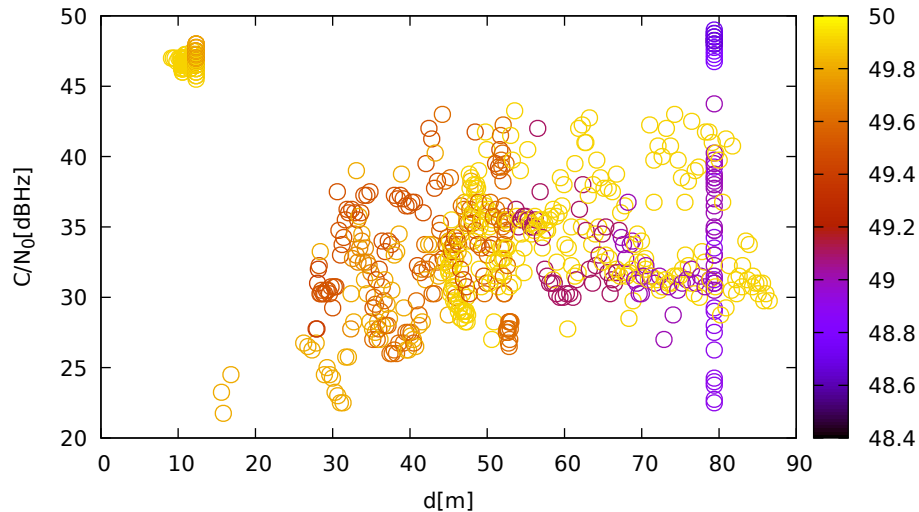
C/N 0 vs distance (JavadLSA at C 3 for G14 at L1)
