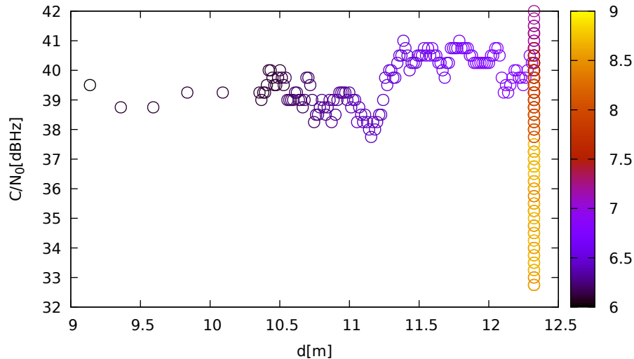
C/N 0 vs distance (JavadLSA at C 3 for G21 at L1)
