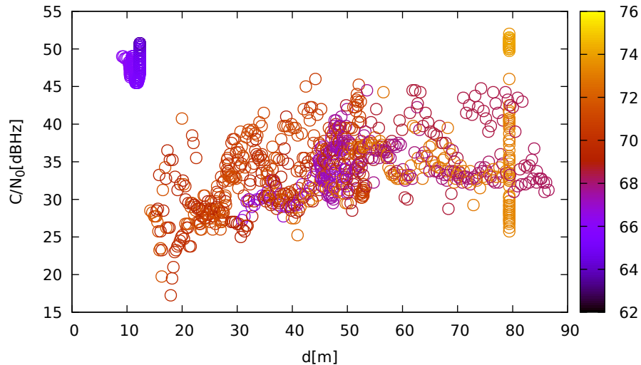
C/N 0 vs distance (JavadLSA at C 3 for G22 at L1)
