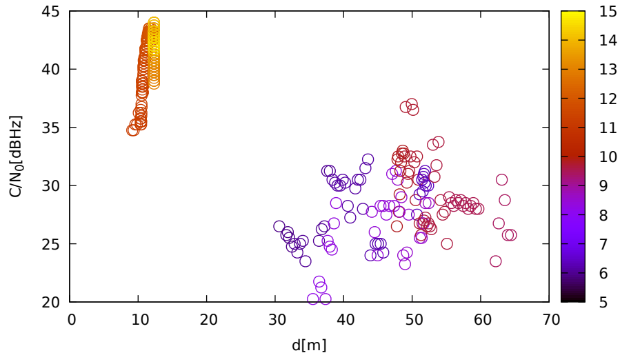
C/N 0 vs distance (JavadLSA at C 3 for G27 at L1)
