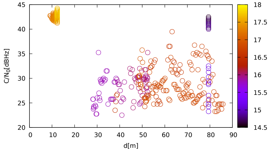
C/N 0 vs distance (JavadLSA at C 3 for G28 at L1)
