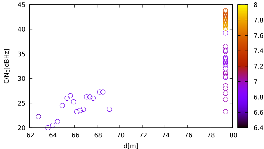
C/N 0 vs distance (JavadLSA at C 3 for G31 at L1)
