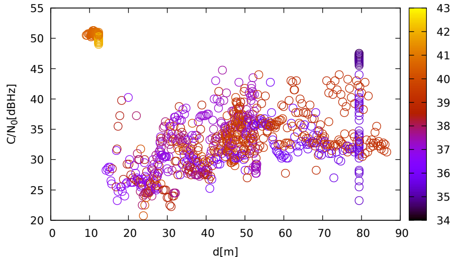
C/N 0 vs distance (JavadLSA at C 3 for G32 at L1)
