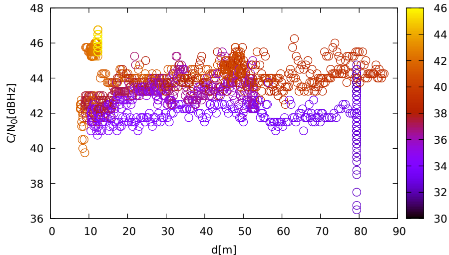
C/N 0 vs distance (JavadLSA at C 3 for R06 at L1)
