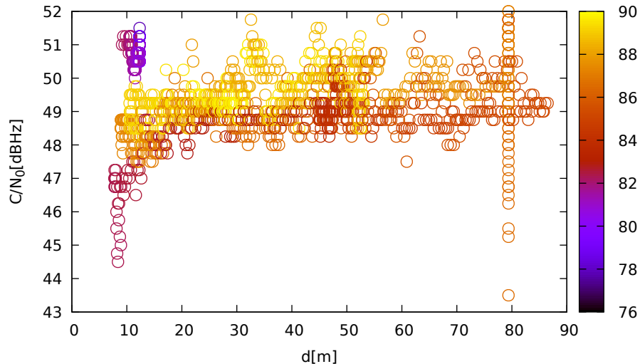
C/N 0 vs distance (JavadLSA at C 3 for R07 at L1)
