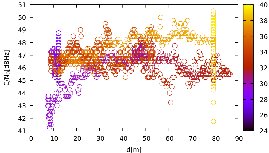
C/N 0 vs distance (JavadLSA at C 3 for R08 at L1)
