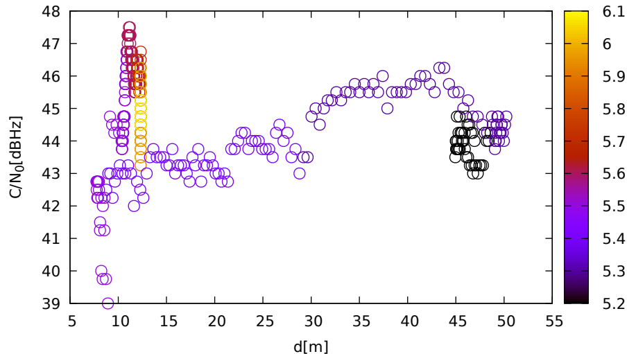
C/N 0 vs distance (JavadLSA at C 3 for R14 at L1)
