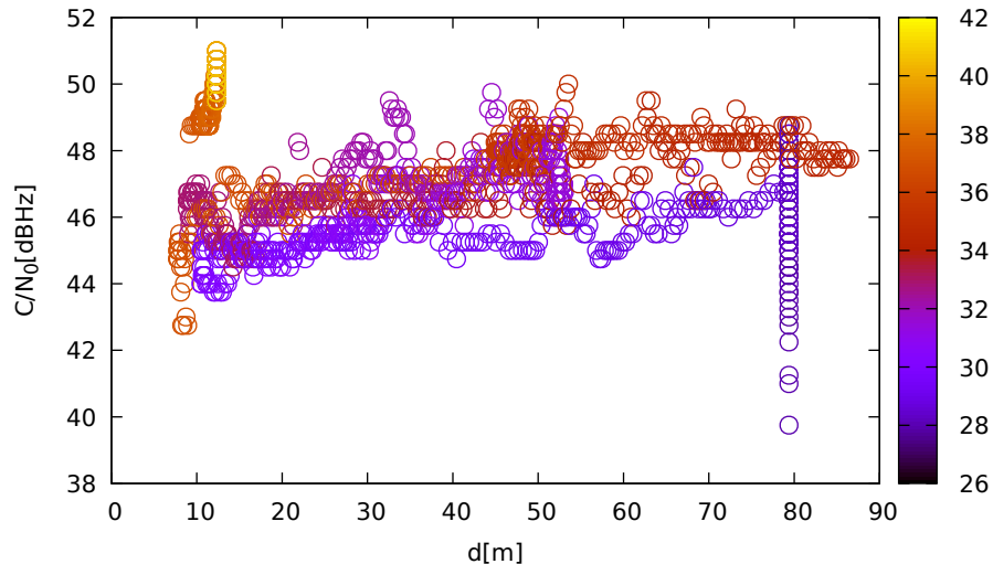
C/N 0 vs distance (JavadLSA at C 3 for R21 at L1)
