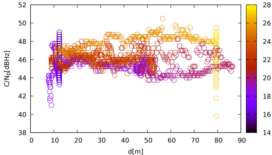
C/N 0 vs distance (JavadLSA at C 3 for R23 at L1)
