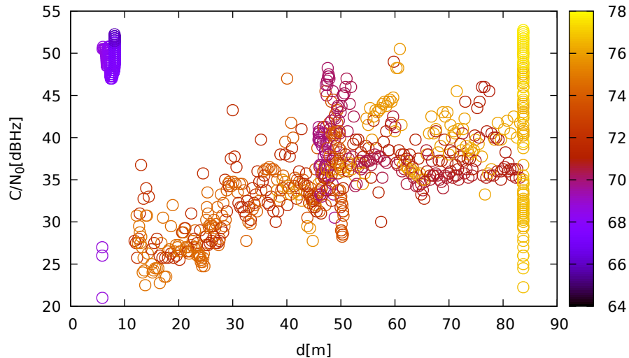
C/N 0 vs distance (JavadVS at C 3 for G01 at L1)
