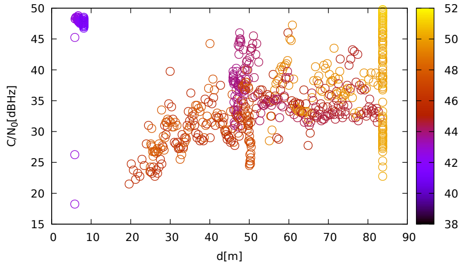
C/N 0 vs distance (JavadVS at C 3 for G03 at L1)
