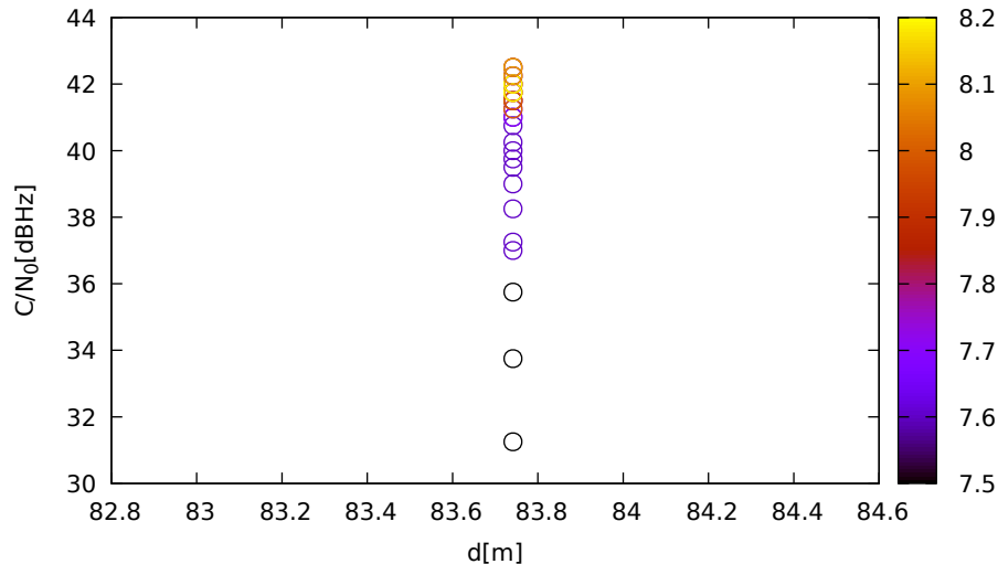
C/N 0 vs distance (JavadVS at C 3 for G04 at L1)
