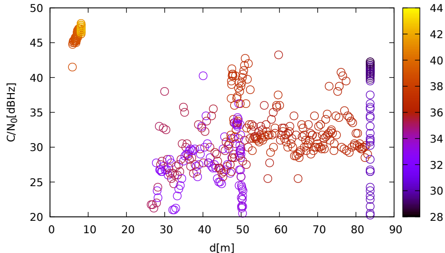
C/N 0 vs distance (JavadVS at C 3 for G08 at L1)
