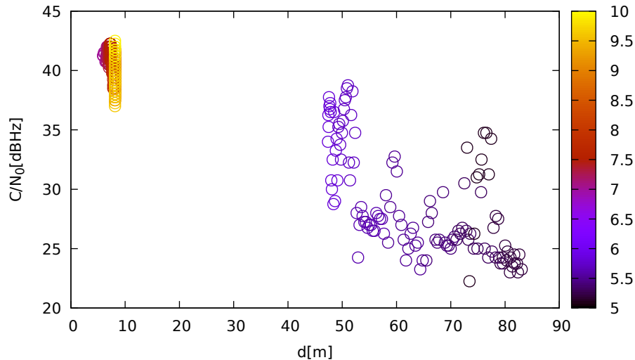
C/N 0 vs distance (JavadVS at C 3 for G10 at L1)
