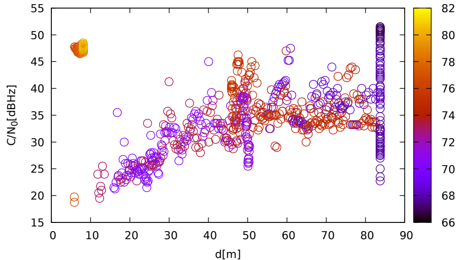
C/N 0 vs distance (JavadVS at C 3 for G11 at L1)
