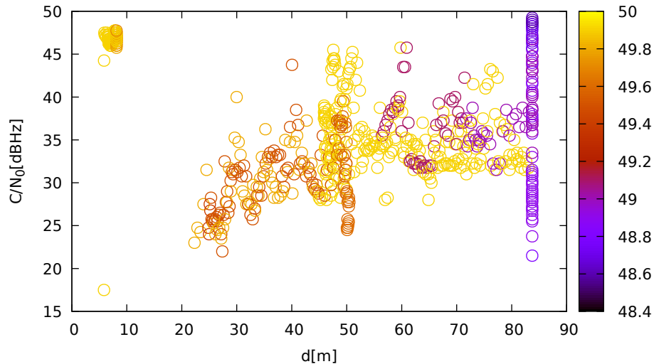
C/N 0 vs distance (JavadVS at C 3 for G14 at L1)
