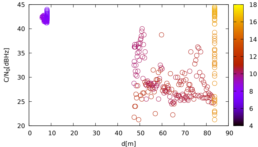
C/N 0 vs distance (JavadVS at C 3 for G17 at L1)
