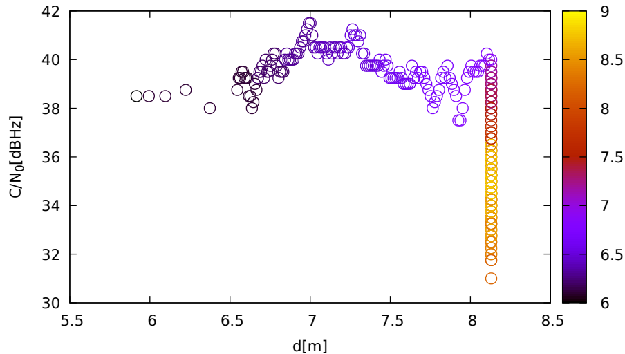
C/N 0 vs distance (JavadVS at C 3 for G21 at L1)
