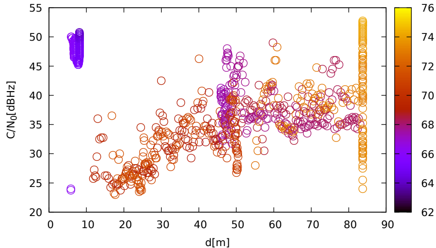
C/N 0 vs distance (JavadVS at C 3 for G22 at L1)
