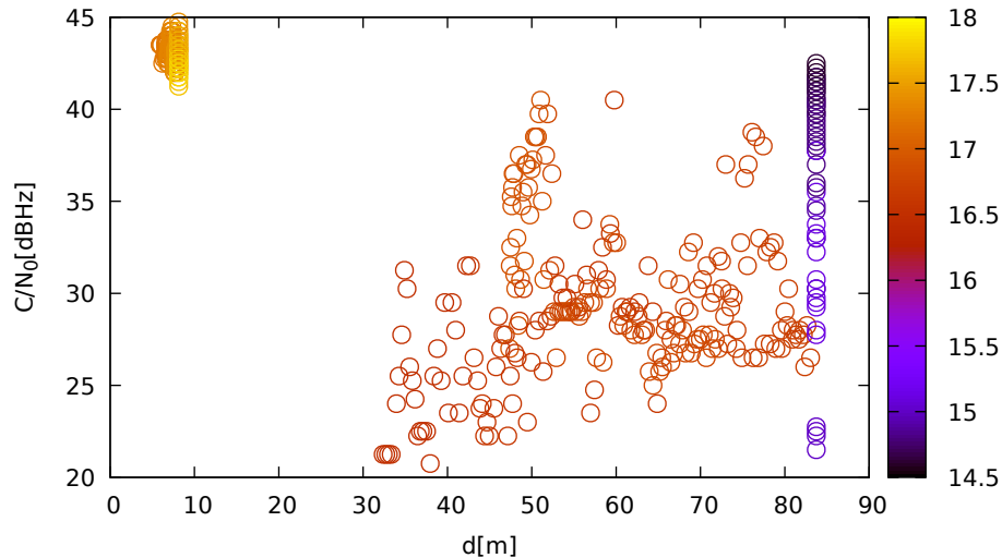
C/N 0 vs distance (JavadVS at C 3 for G28 at L1)
