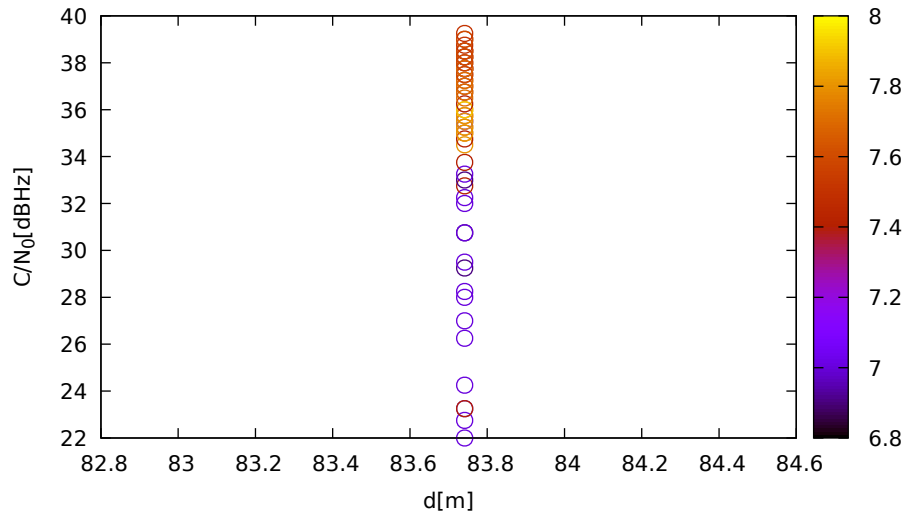
C/N 0 vs distance (JavadVS at C 3 for G31 at L1)
