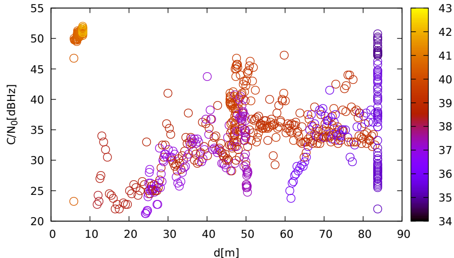
C/N 0 vs distance (JavadVS at C 3 for G32 at L1)
