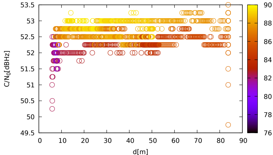
C/N 0 vs distance (JavadVS at C 3 for R07 at L1)
