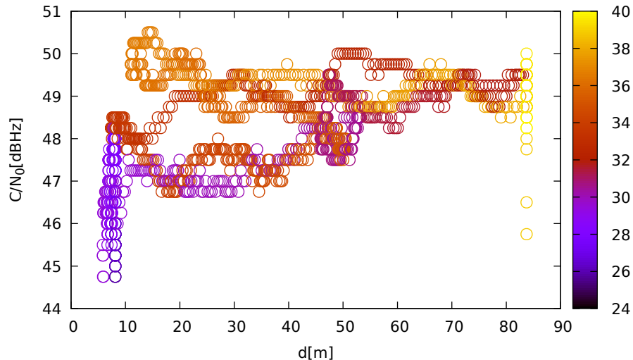
C/N 0 vs distance (JavadVS at C 3 for R08 at L1)
