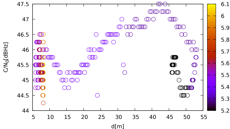
C/N 0 vs distance (JavadVS at C 3 for R14 at L1)
