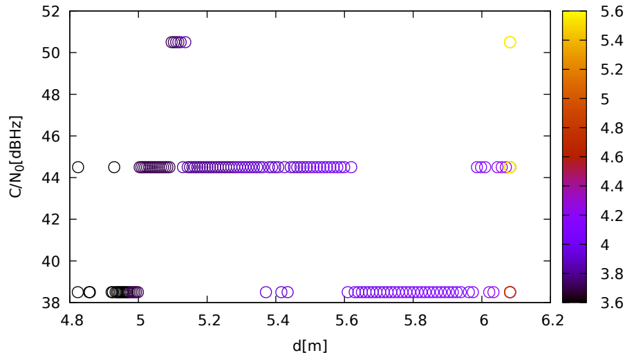
C/N 0 vs distance (LeicaGS15 at C 3 for E02 at L1)
