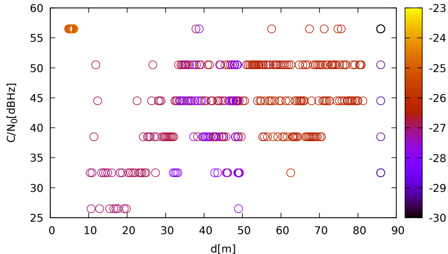
C/N 0 vs distance (LeicaGS15 at C 3 for E04 at L1)
