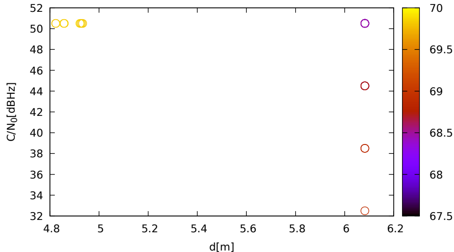
C/N 0 vs distance (LeicaGS15 at C 3 for E05 at L1)
