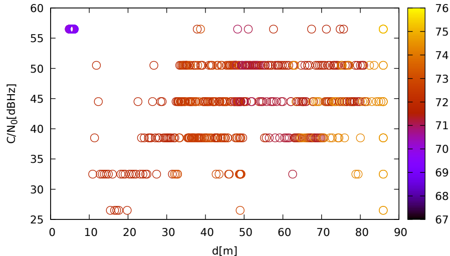
C/N 0 vs distance (LeicaGS15 at C 3 for E09 at L1)
