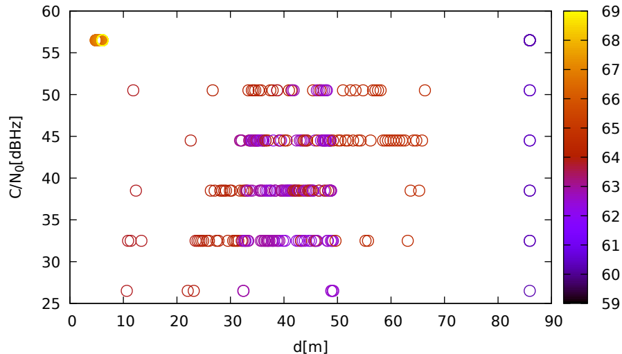
C/N 0 vs distance (LeicaGS15 at C 3 for E11 at L1)
