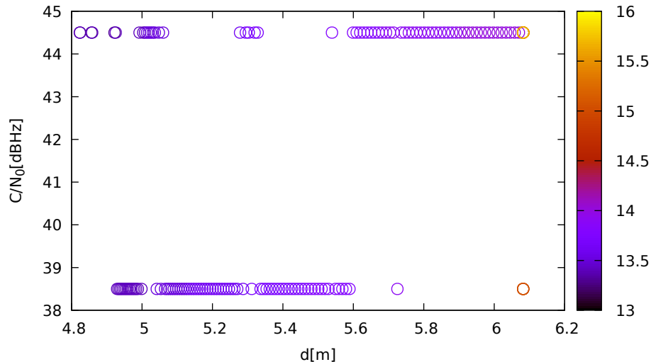
C/N 0 vs distance (LeicaGS15 at C 3 for E12 at L1)
