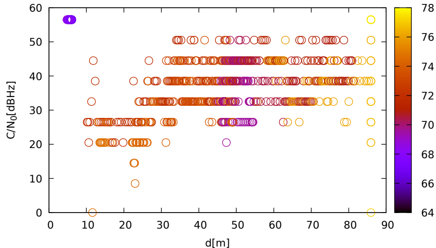
C/N 0 vs distance (LeicaGS15 at C 3 for G01 at L1)
