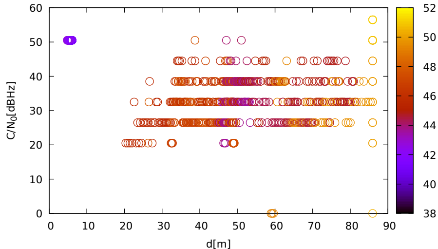
C/N 0 vs distance (LeicaGS15 at C 3 for G03 at L1)
