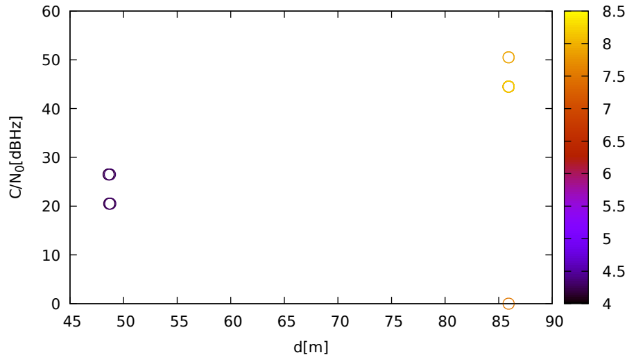
C/N 0 vs distance (LeicaGS15 at C 3 for G04 at L1)
