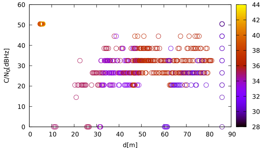
C/N 0 vs distance (LeicaGS15 at C 3 for G08 at L1)
