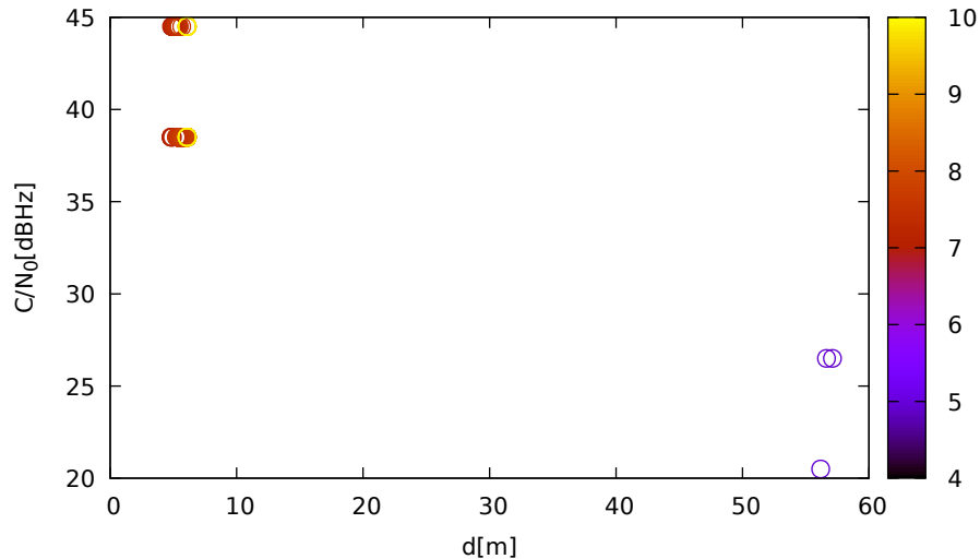
C/N 0 vs distance (LeicaGS15 at C 3 for G10 at L1)
