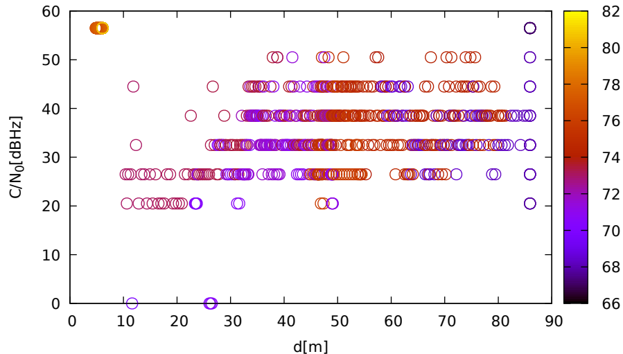
C/N 0 vs distance (LeicaGS15 at C 3 for G11 at L1)
