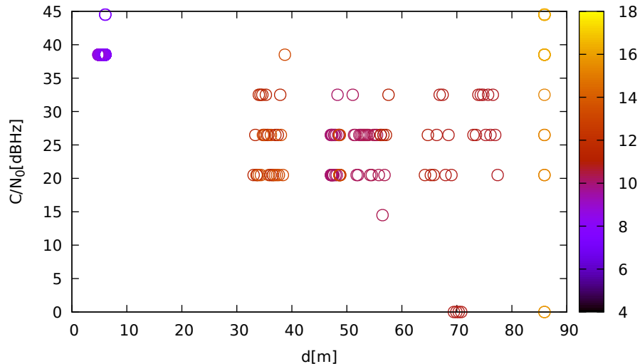
C/N 0 vs distance (LeicaGS15 at C 3 for G17 at L1)
