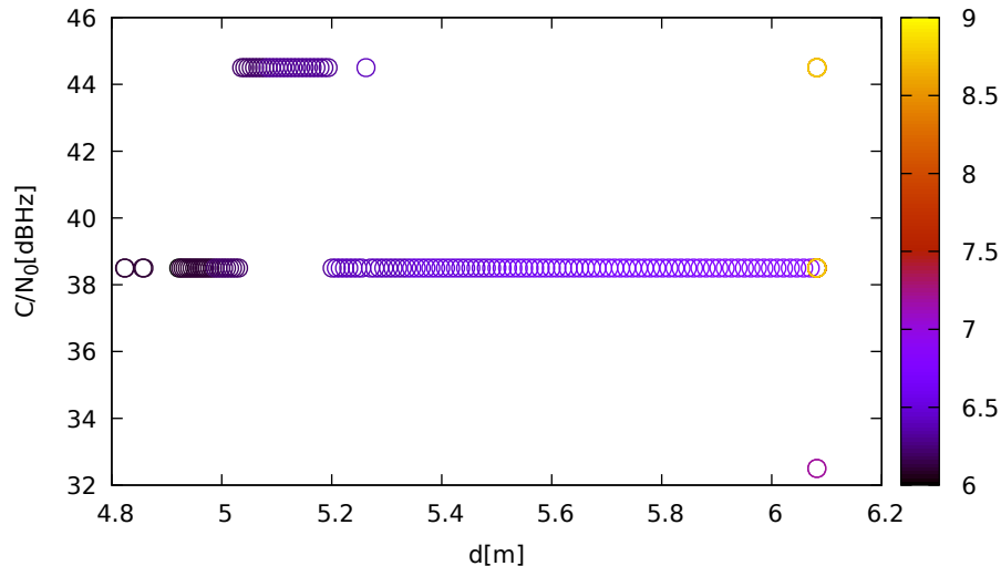
C/N 0 vs distance (LeicaGS15 at C 3 for G21 at L1)
