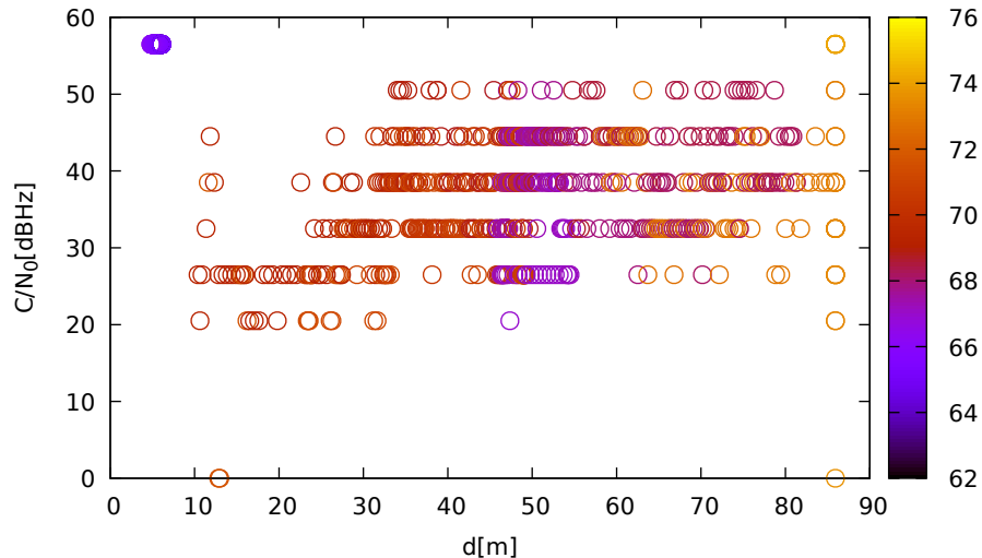
C/N 0 vs distance (LeicaGS15 at C 3 for G22 at L1)
