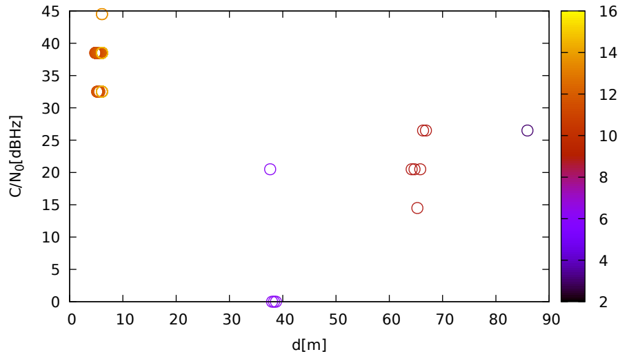
C/N 0 vs distance (LeicaGS15 at C 3 for G27 at L1)
