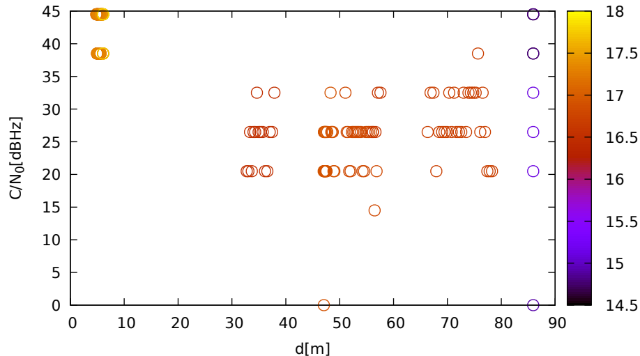
C/N 0 vs distance (LeicaGS15 at C 3 for G28 at L1)
