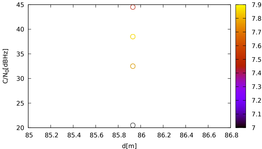
C/N 0 vs distance (LeicaGS15 at C 3 for G31 at L1)
